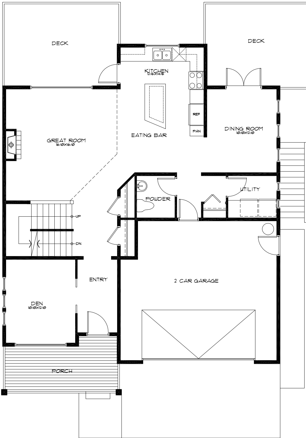
1 A2.2 MAIN FLOOR PLAN Scale 1/4" = 1'-0" MAIN FLOOR 1167 SQ. FT GARAGE 460 SQ. FT
